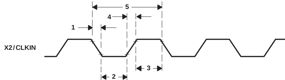
Figure 7. X2/CLKIN Timing
